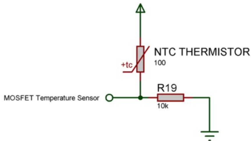
Figure 3.7: CIRCUIT DIAGRAM OF TEMPERATURE SENSOR
