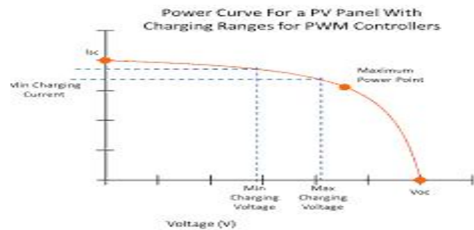
Figure 2.2: PWM SOLAR I-V AND POWER CURVES
