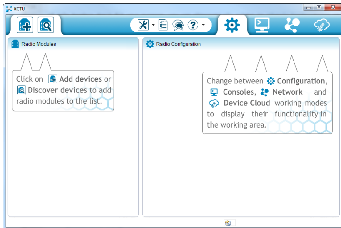
Figure 3.2: software interface
