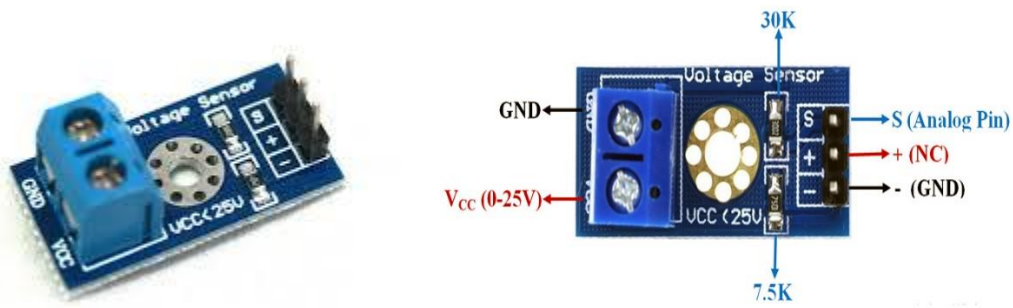
FIGURE 3.3: VOLTAGE SENSORS
