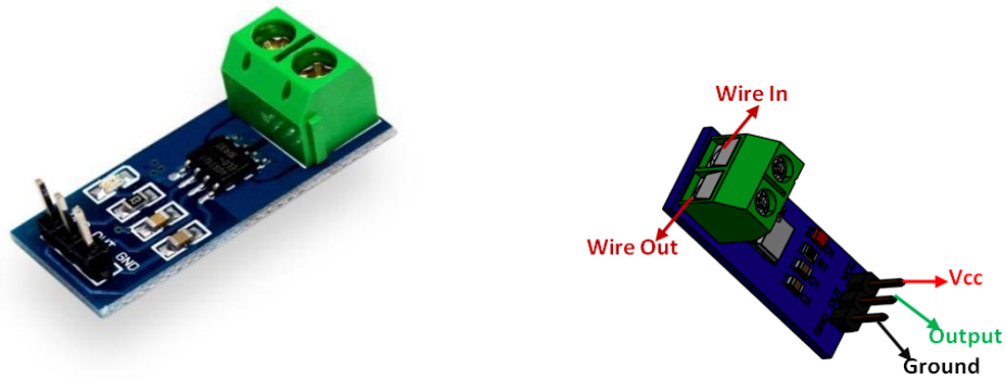
FIGURE 3.4: CURRENT SENSORS
