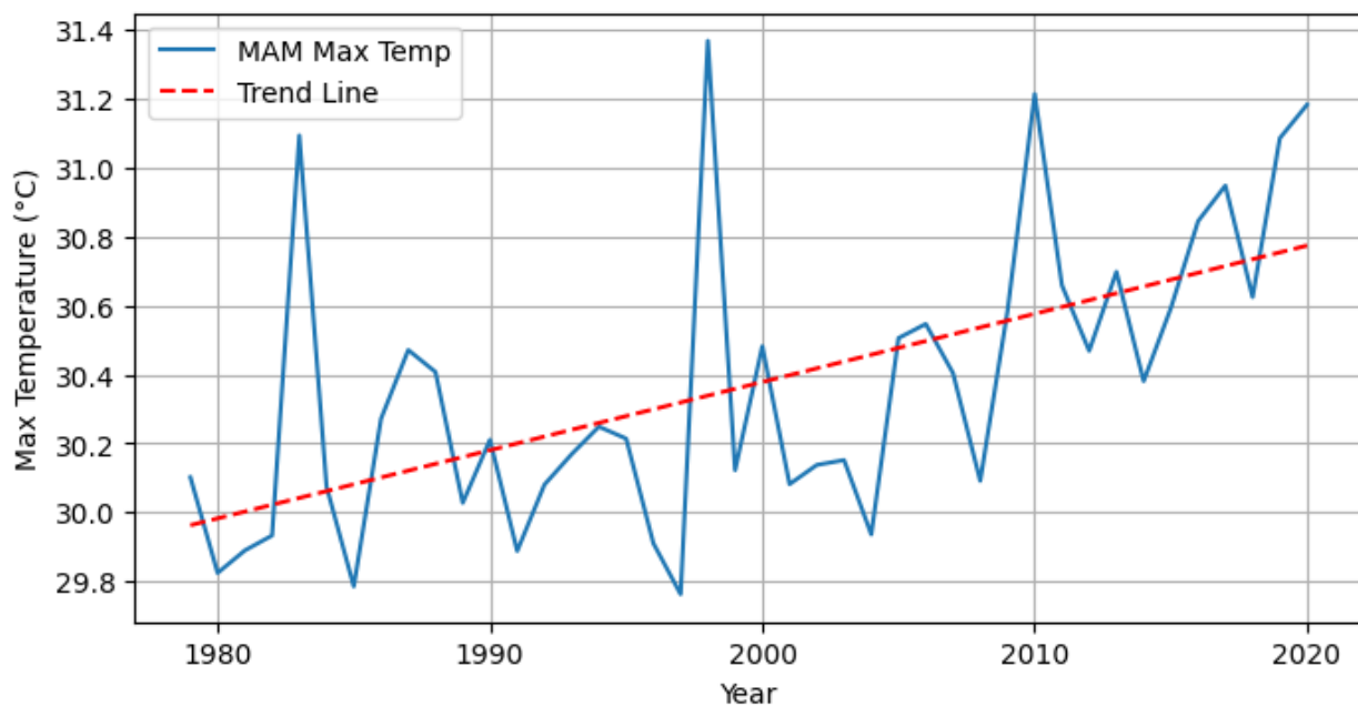
Figure 4.58: Maximum Temperature Data for MAM Season
