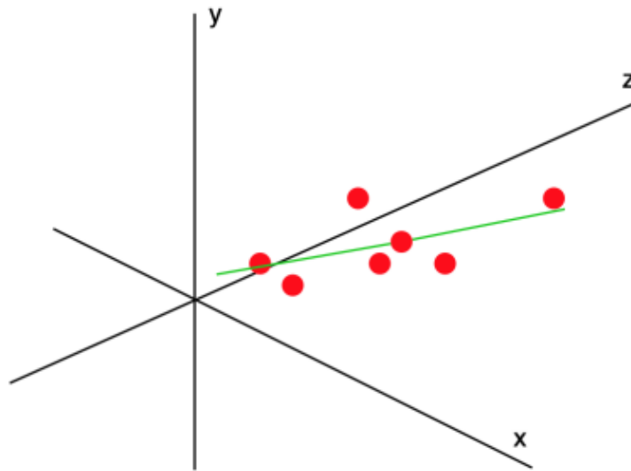
Figure 2.20: Multilinear regression
