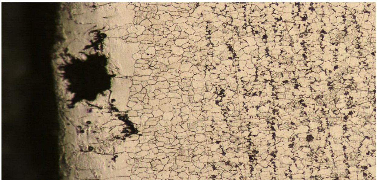
Figure 4.11: Evidence of thermal oxidation on the tube ID.
