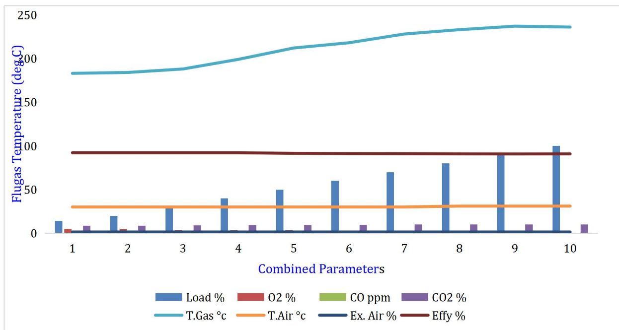
Figure 4.25: Relationship between flue gas parameters and boiler loads
