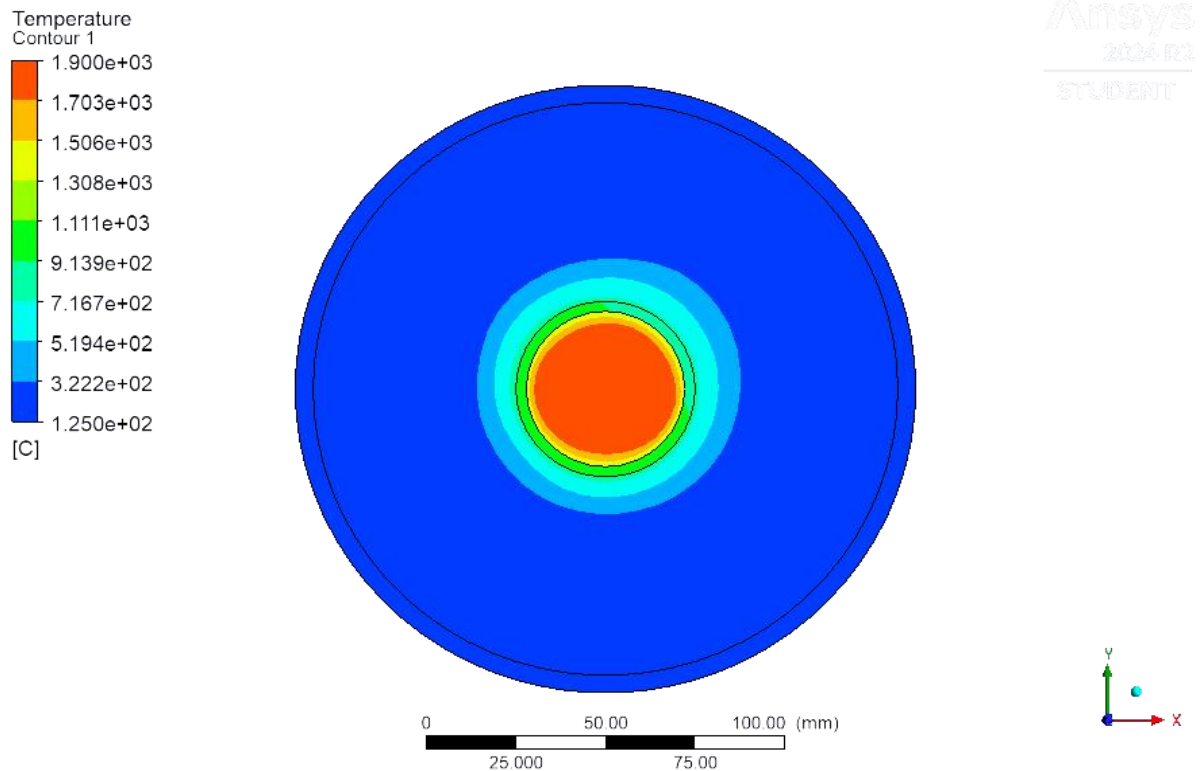
Figure 4.13: Distribution of Temperature for Scale Free Condition for Natural Gas
