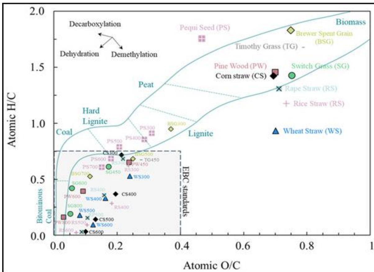
Fig. 2.4: Van Krevelen's diagram of the H/C to O/C ratio (Source: Silveira et al. , 2023).
