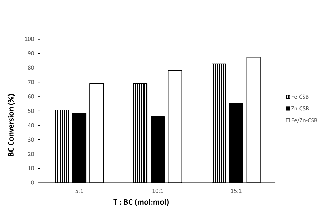
Fig. 4.29: Effect of Mole Ratio of T:BC on Benzyltoluene over Metal - Doped Catalyst (Catalyst Loading 8.2 wt% BC, Temperature 70°C, Time, 180 min)
