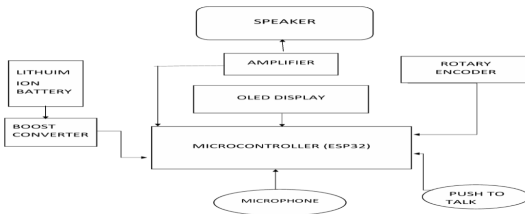
Figure 1.1: Block Diagram
