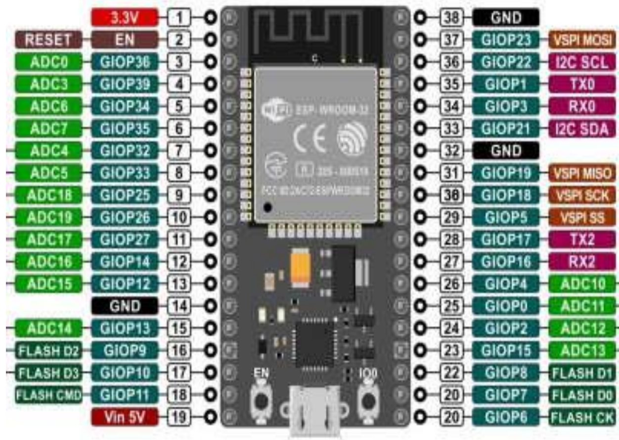
Figure 2.4.1: ESP microcontroller
