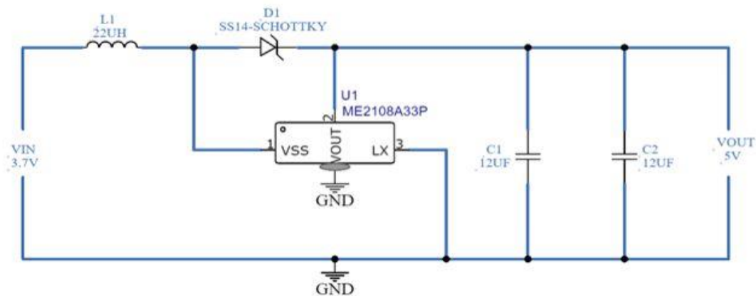
Figure 3.1: The overview of the boost converter
