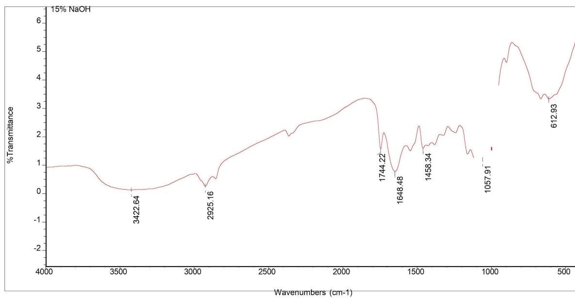
Fig. 4.5. 15% NaOH Peaks
