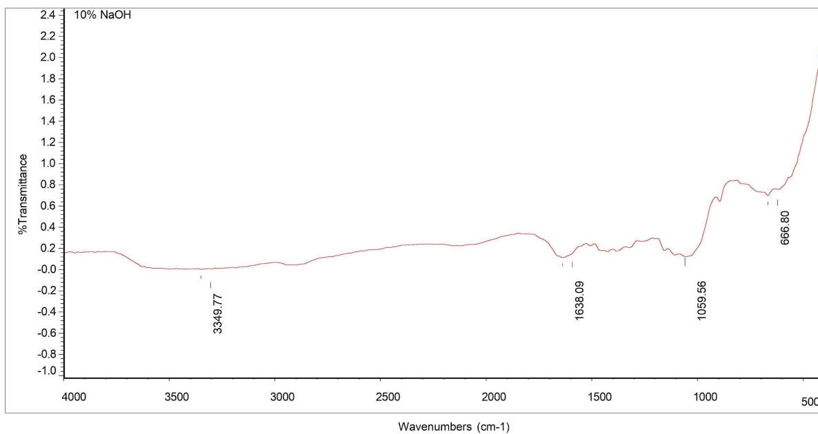
Fig. 4.6. 10% NaOH Peaks
