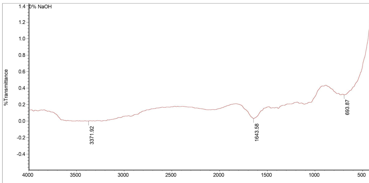
Fig. 4.1. 0% NaOH Peaks
