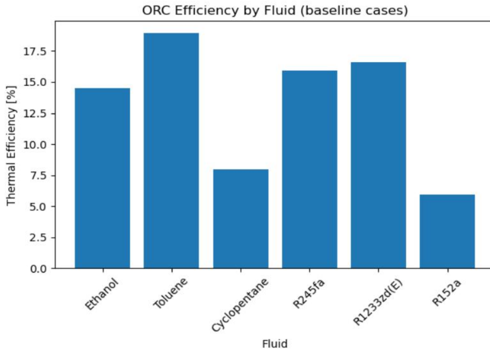
Figure 4.1 Bar chart showing efficiency and ORC fluids.
