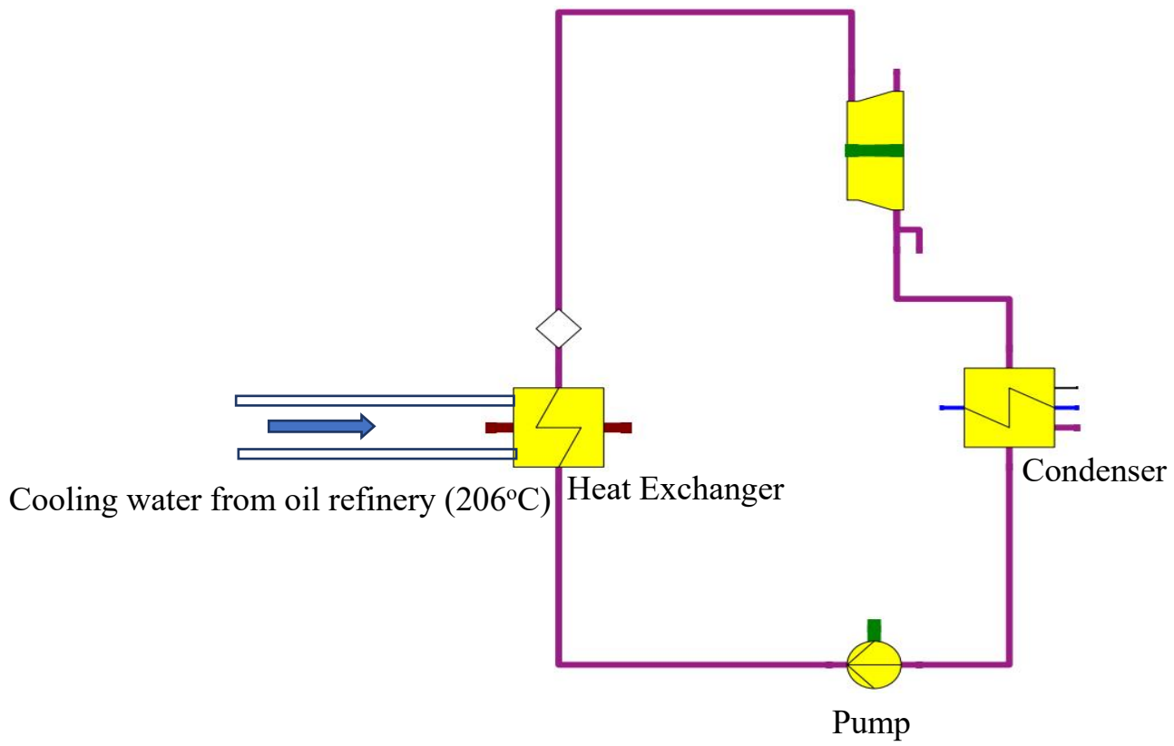
Figure 3.1 Schematic layout of ORC system
