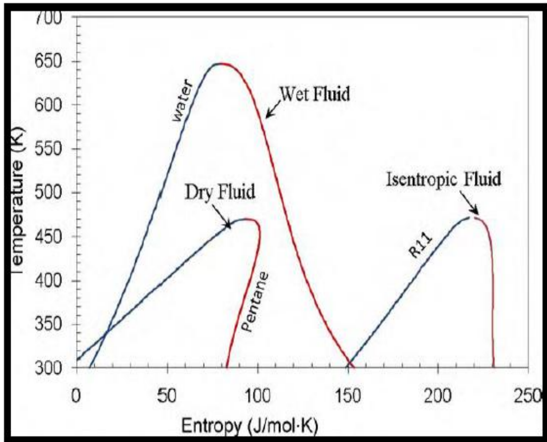
Figure 2.2: T-s diagram for Wet, Isentropic and Dry fluids.
