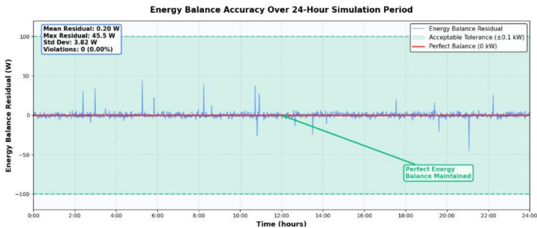
Figure 4.6: Energy Balance Residual Over 24-Hour Simulation Period
