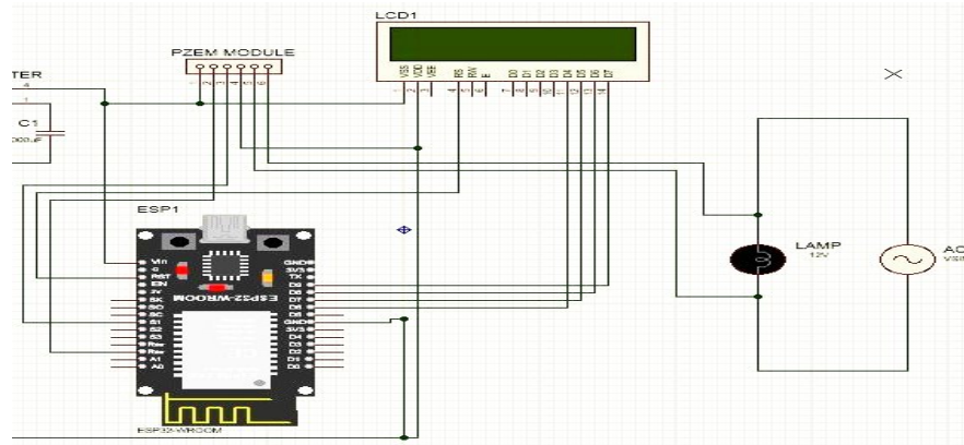
Fig 3.9: ESP32 Dev module with the PZEM-004T module, LCD screen, AC supply unit and external load source.
