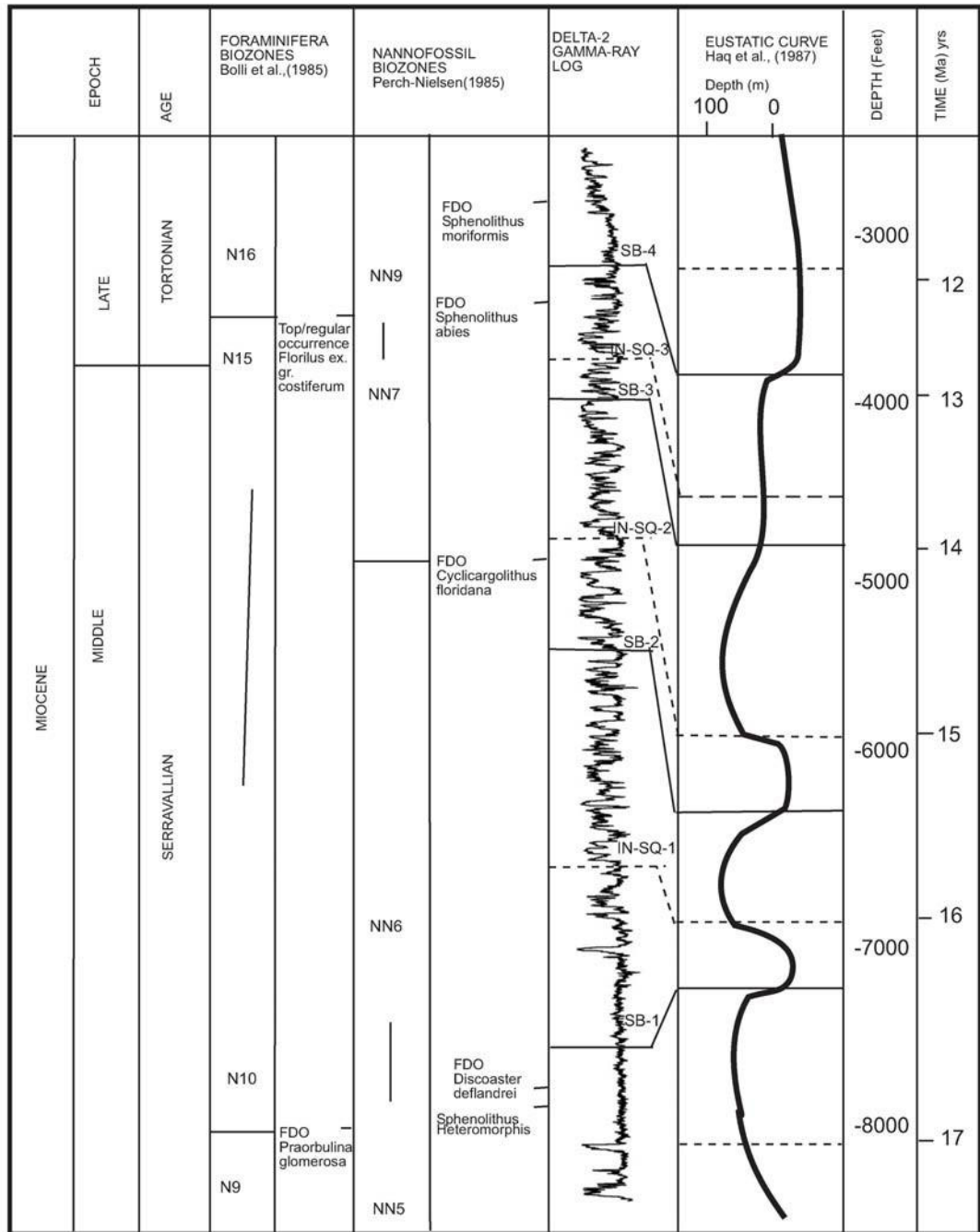
Figure 8. Biostratigraphic zonation within Delta-2 Well. Well log variations are also related to sea level curve of Haq (1987). The age of intra-sequence surfaces in this well estimated from biostrigraphic divisions appear to generally match the date of maximum flooding surfaces on the Haq curve.
