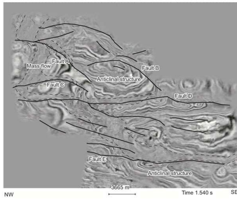
Figure 33. Seismic horizon slice on sequence boundary 2. It shows the interpreted and un-interpreted slices. Submarine mass flow channel entered from the north and cut through the middle fault E to the hanging wall anticlinal structure and exist the slice to the southeast.
