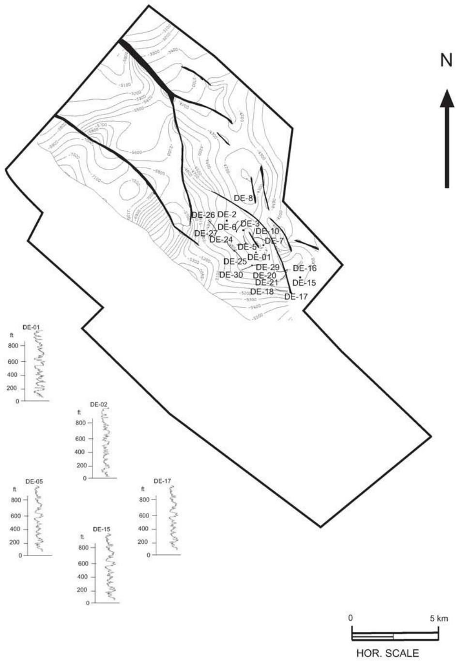
Figure 19. Structure map of intra-sequence 2. Log patterns show an overall aggrading to prograding pattern.
