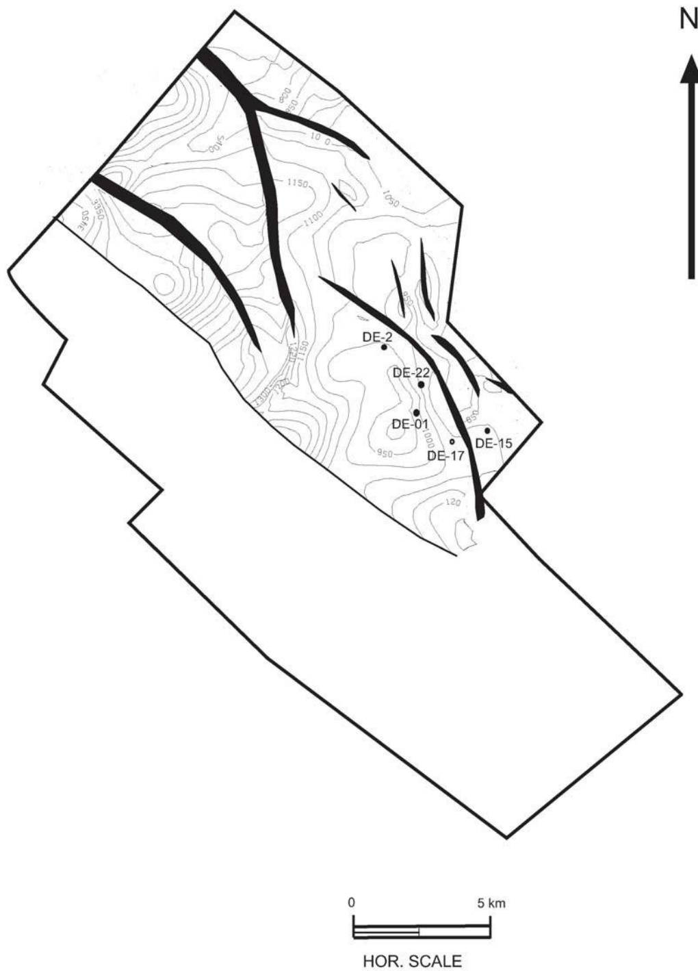
Figure 29. Isolith map between intra-sequence surfaces 2 and 3. It shows nature of growth strata in the hanging walls of the faults.
