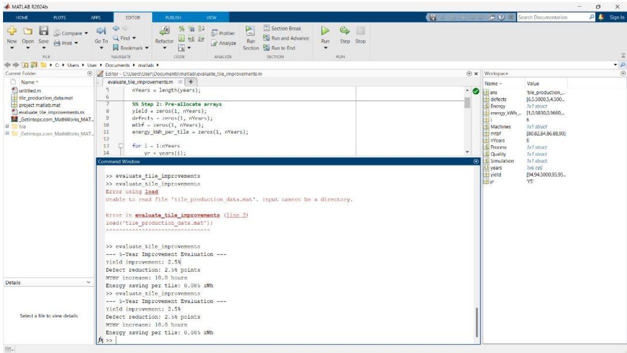
Figure 4.3- MATLAB preview
