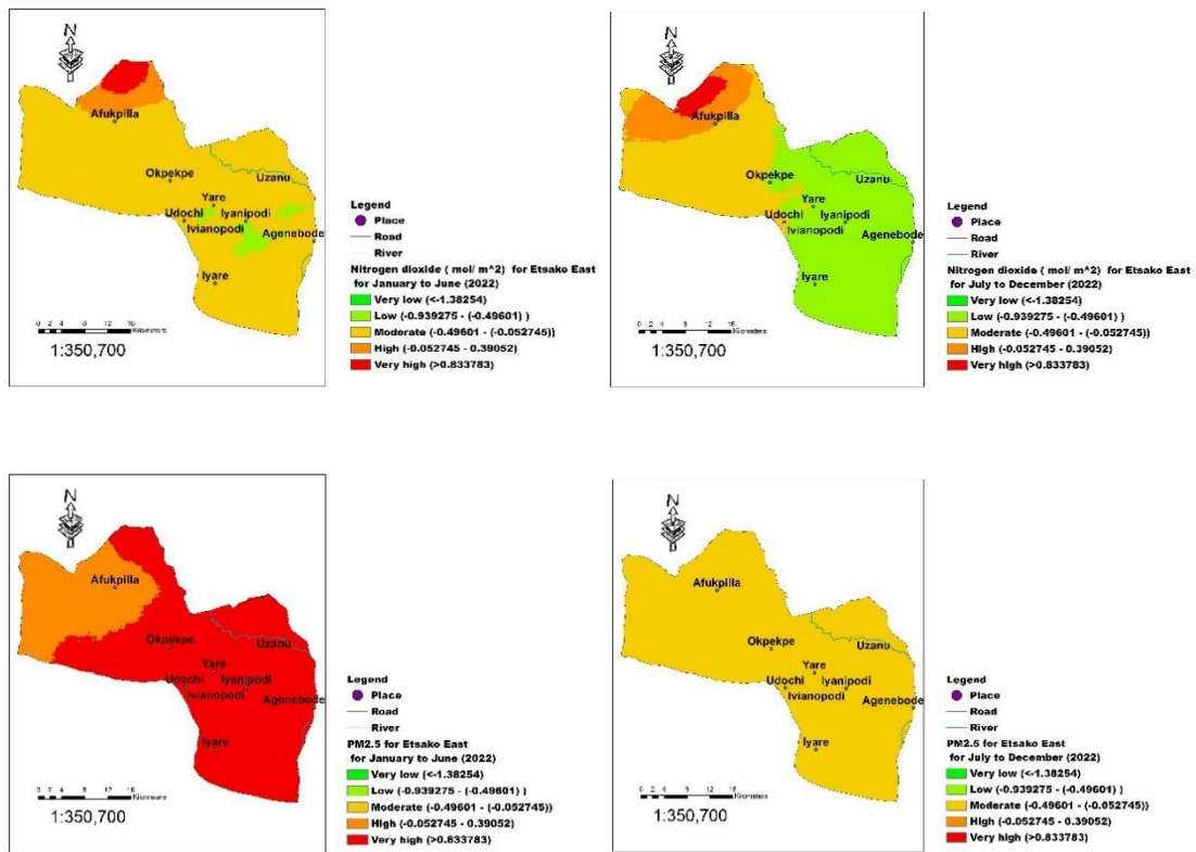
Figure: 4.7. Spatial distribution of \text{NO}_2 and \text{PM}_{2.5} concentration for January to June and July to December 2022
