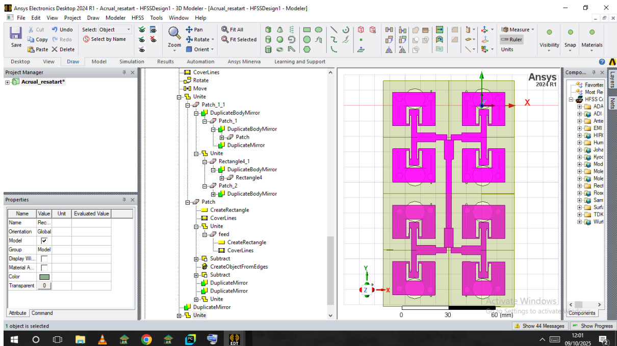
Figure 3.80: 4 \times 2 array
