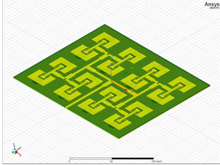
Figure 4.13: 4 \times 4 array with U-slots and DGS.
