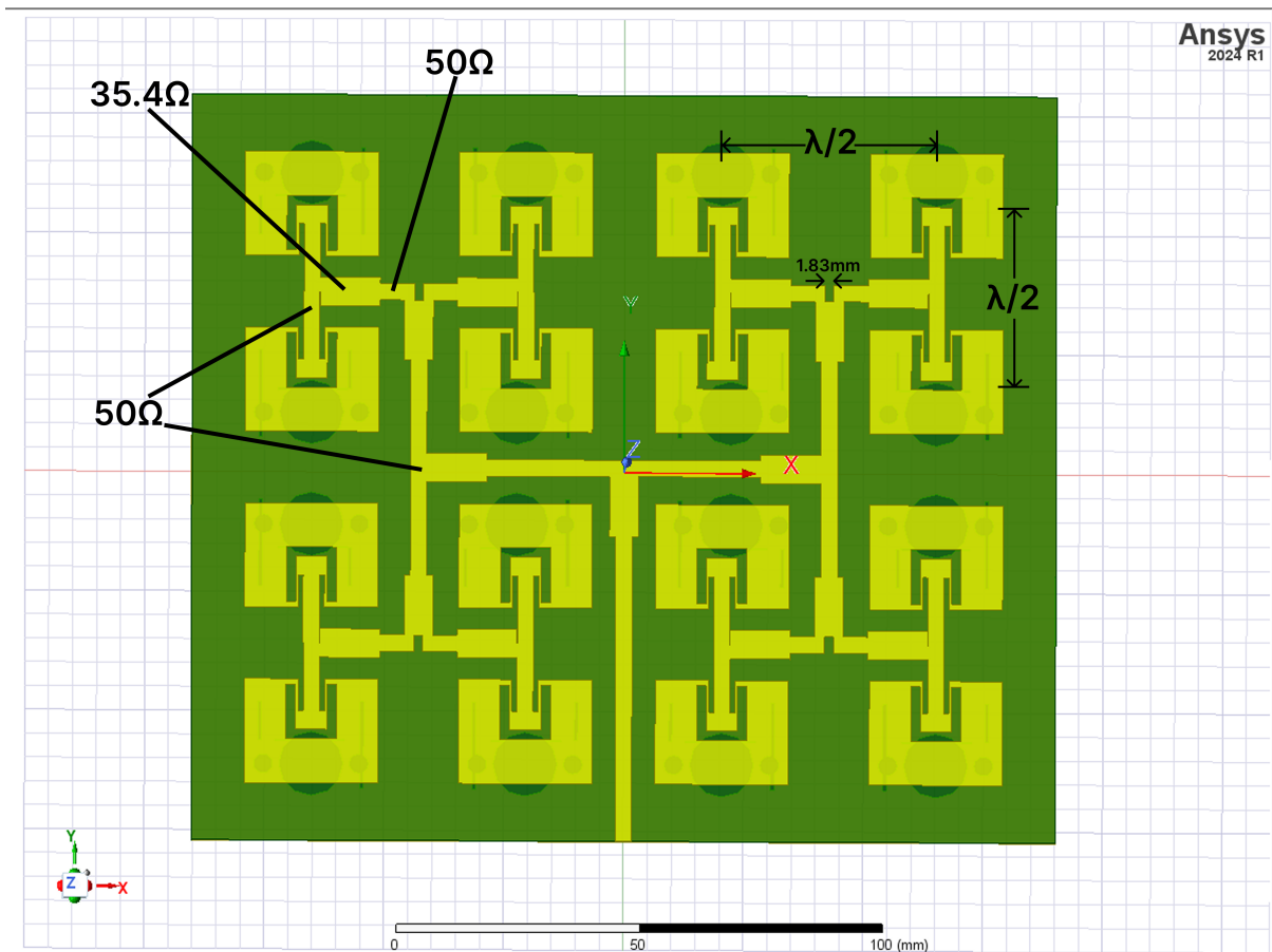
Figure 3.88: Final Array
