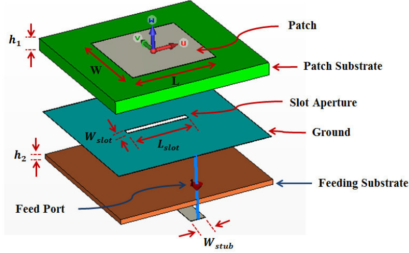
Figure 2.6: A patch antenna with an aperture-coupled feed mechanism (Naji et al. 2012)
