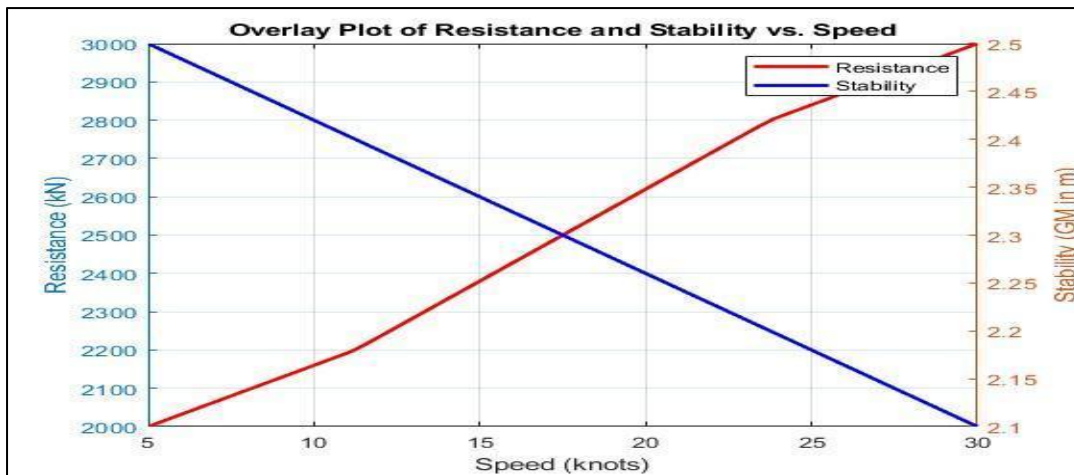
Figure 4.4: Overlay plot of Resistance vs Speed
