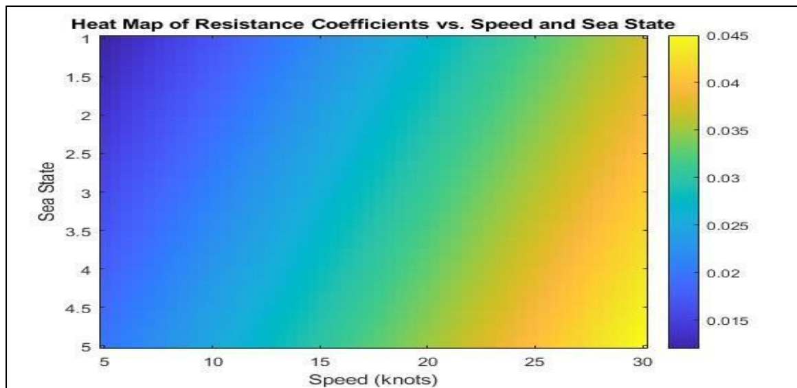
Figure 4.6 illustrates a heat map displaying the variation of wave-making resistance coefficients as a function of ship speed (in knots) and sea state (on an arbitrary scale). The x-axis represents the speed range from 5 to 30 knots, while the y-axis represents the sea state, varying from 1 to 5.
