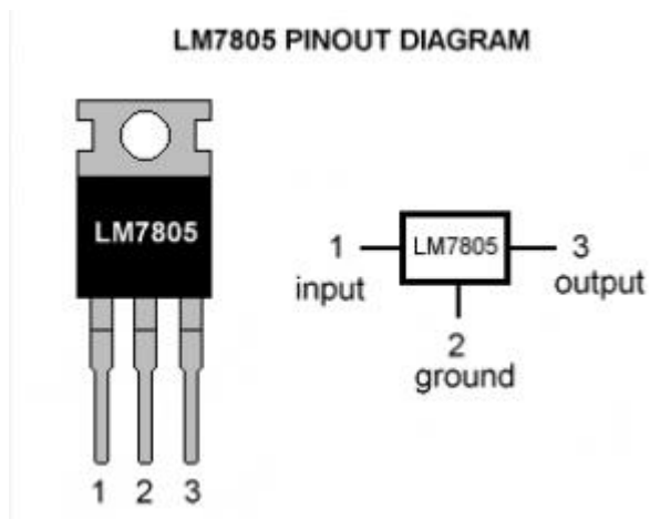
Figure 2.4 Voltage Regulator; U1 7805
