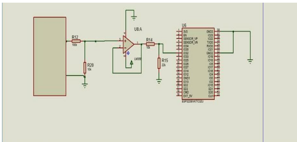
Figure 3.1 Voltage Sensor Circuit.
