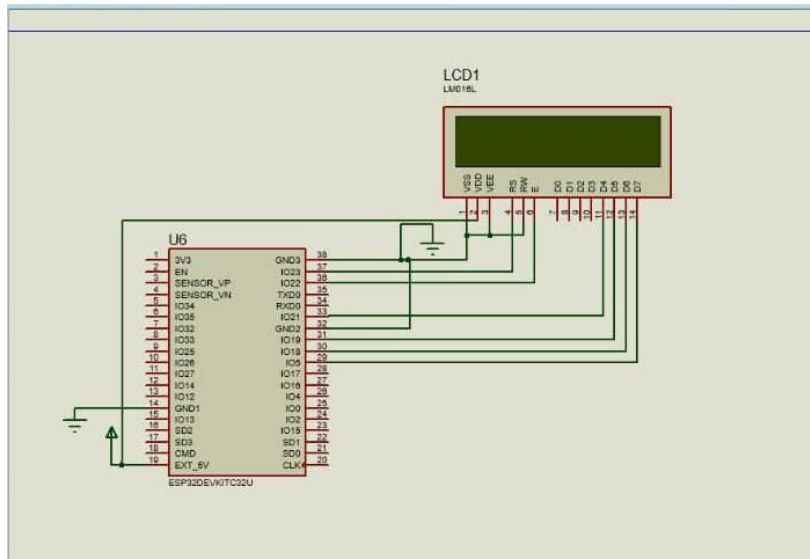
Figure 3.5 LCD Sub-Circuit
