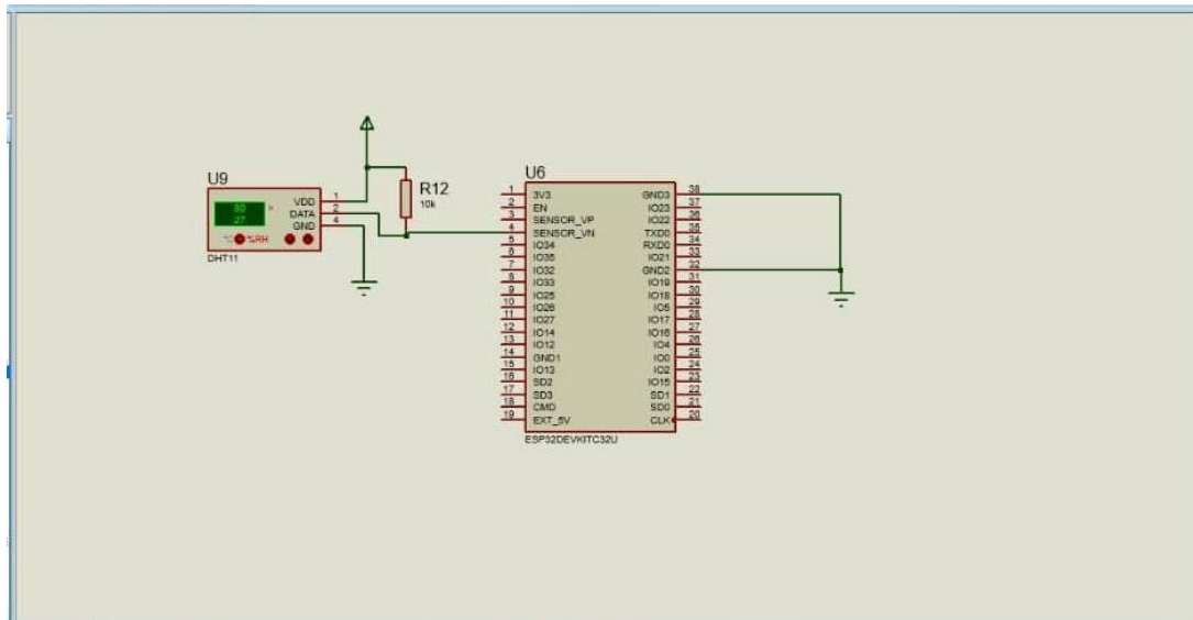
Figure 3.4 DHT11 Sub-Circuit
