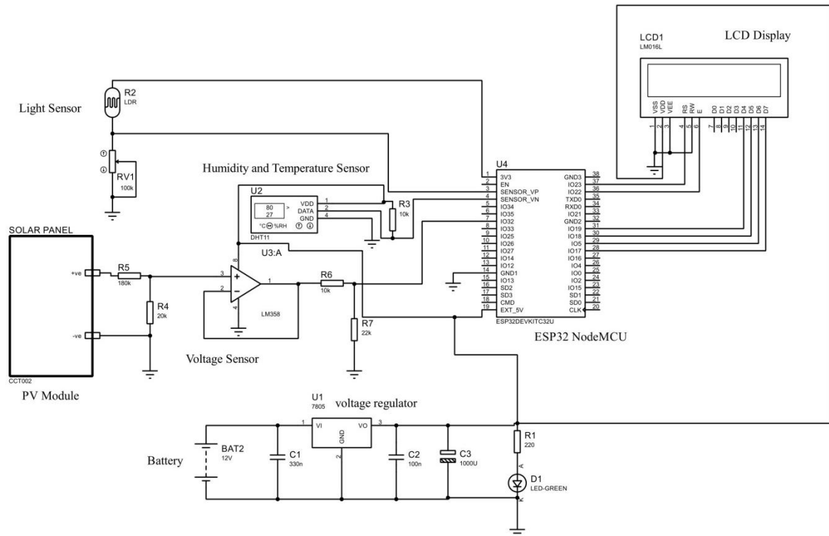
Figure 3.7 Circuit Diagram of A Remote PV Monitoring System
