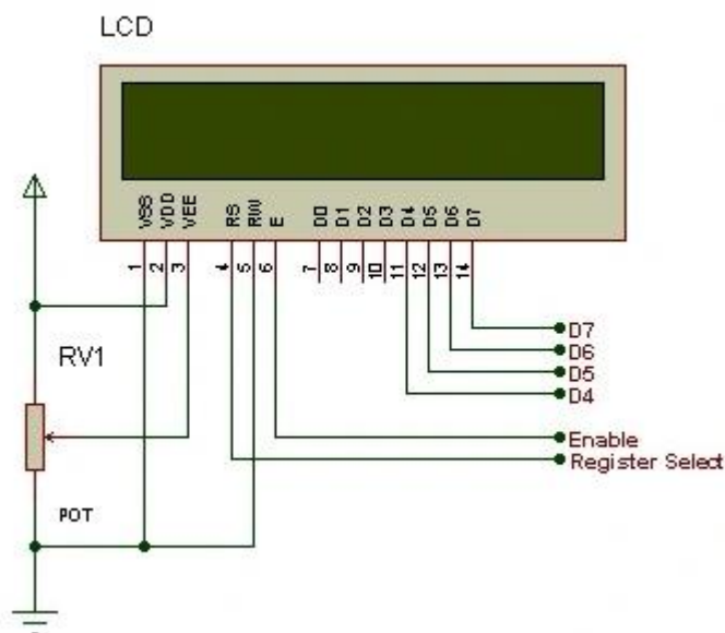
Figure 2.3 LCD1 LM016L
