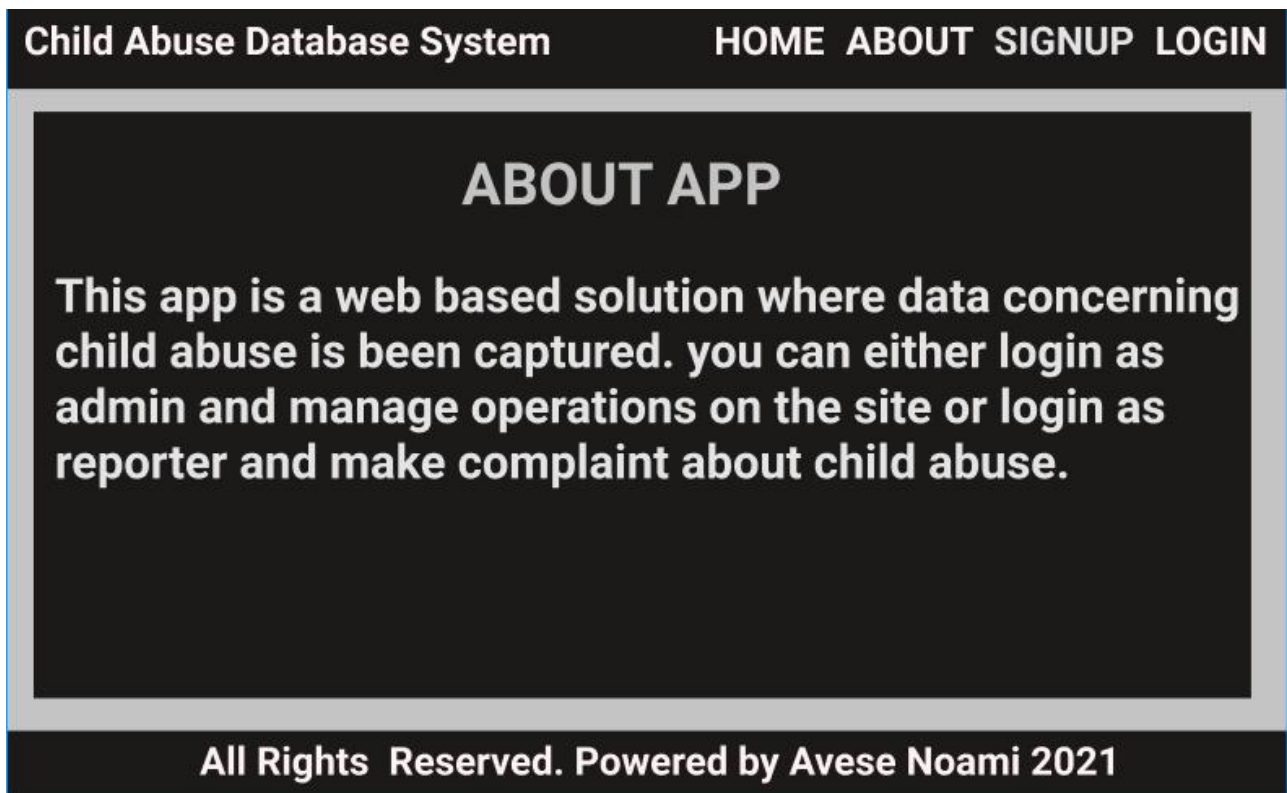
Figure 4.2 About Page
