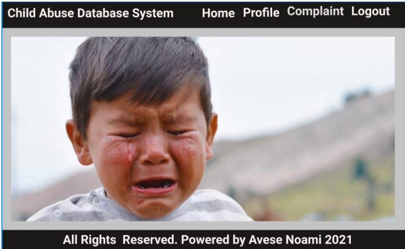
Figure 4.5 Reporter Dashboard
