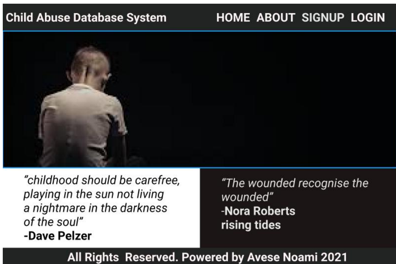
Figure 4.1 Homepage
