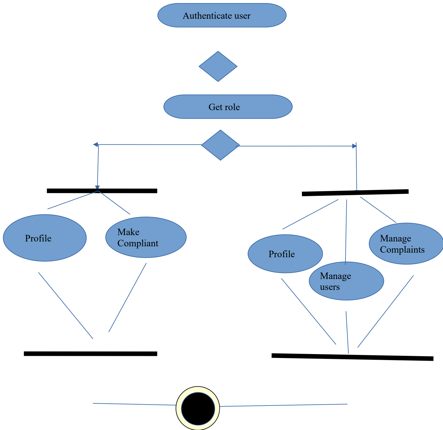
Figure 3.5 Activity diagram for the child abuse database system
