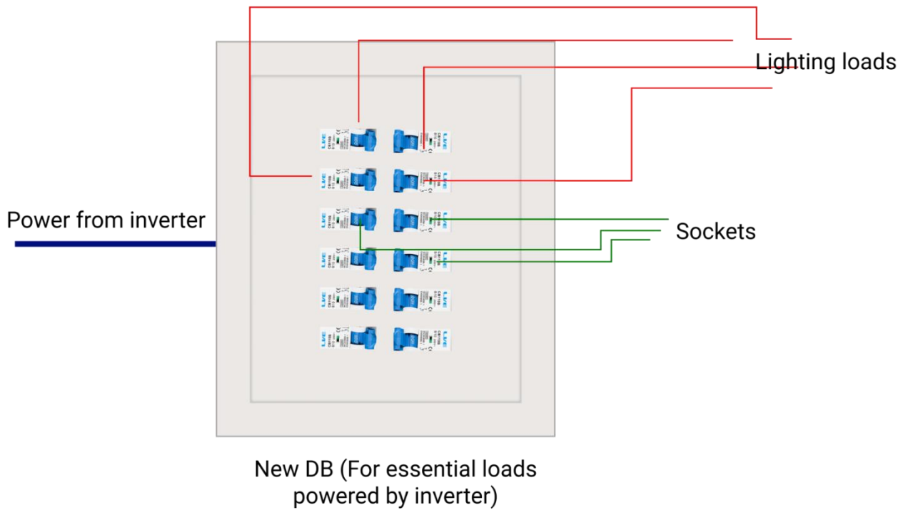
Figure 3.3 New DB (For essential loads powered by inverter)
