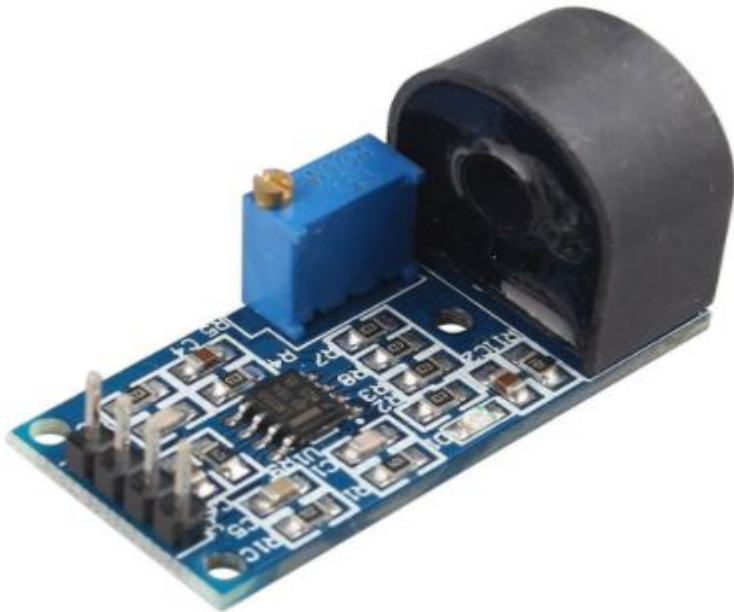
Figure 2.9 LMC358
