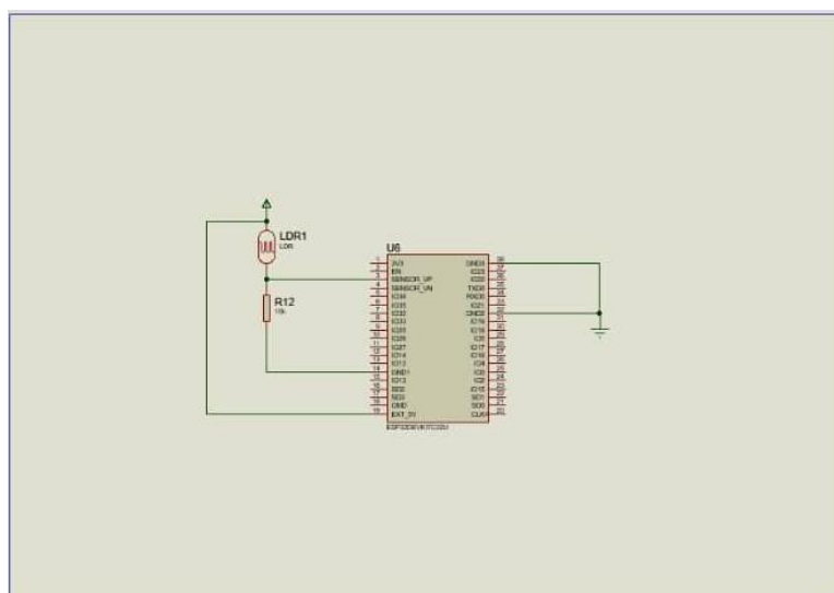
Figure 3.3 LDR Sub-Circuit
