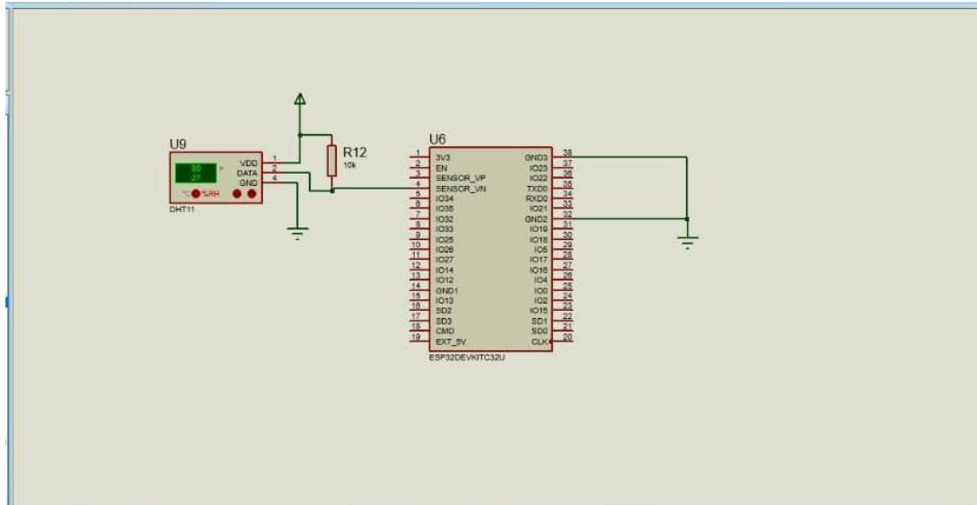
Figure 3.4 DHT11 Sub-Circuit
