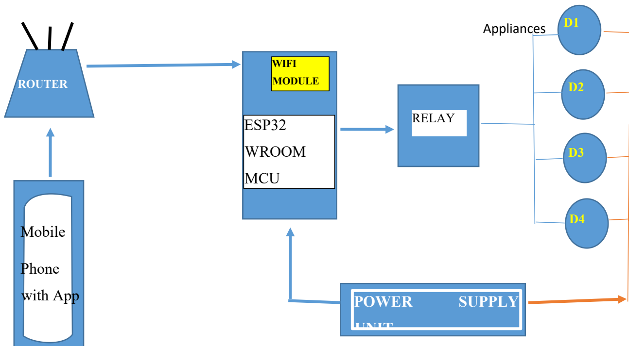
Fig.3.1-Block diagram of the smart home automation system
