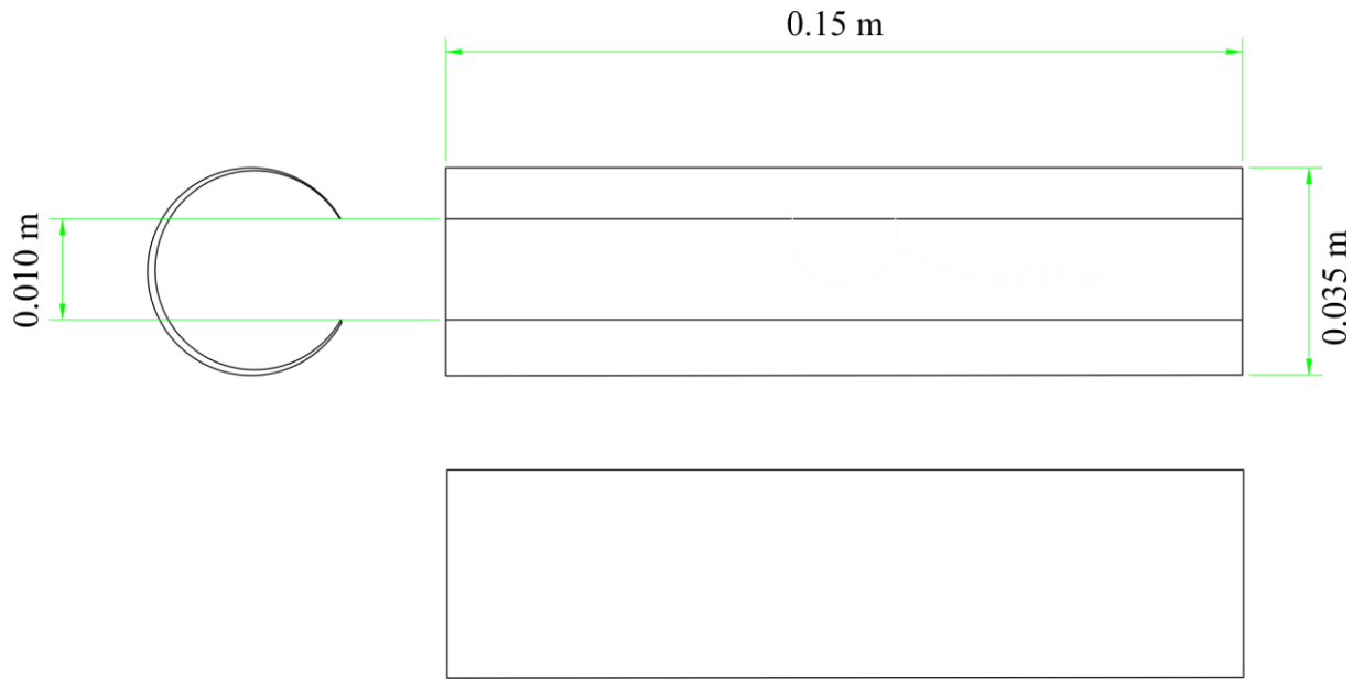
Figure 3.20 – Orthographic view of Agitator Mechanism
