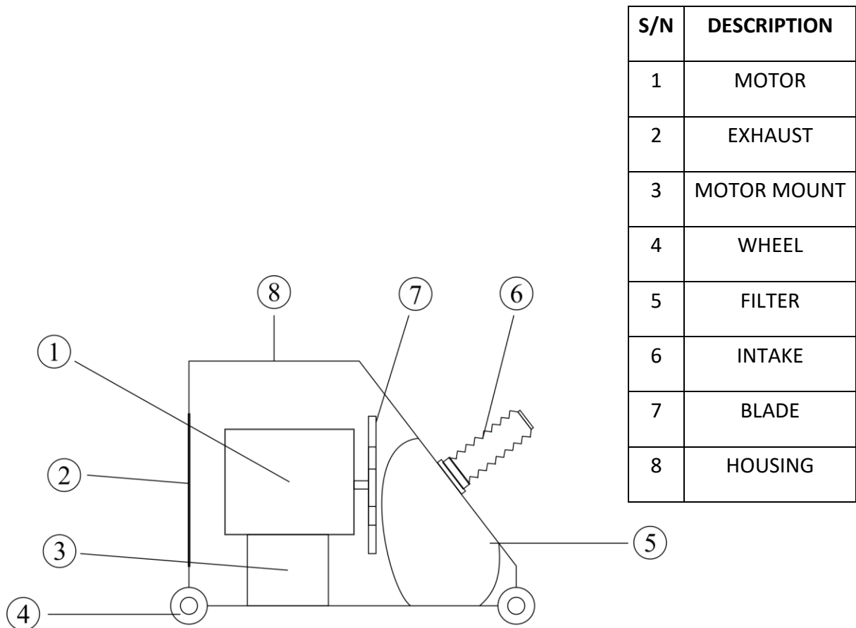
Figure 3.4 – Diagram of design concept three
