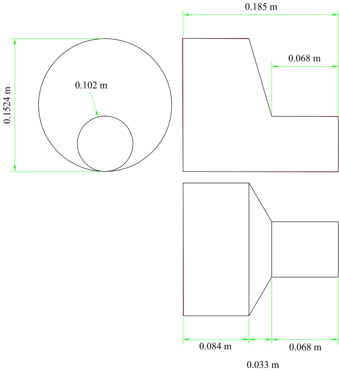
Figure 3.22 – Orthographic view of 6 to 4 Inches Pipe reduction Joint
