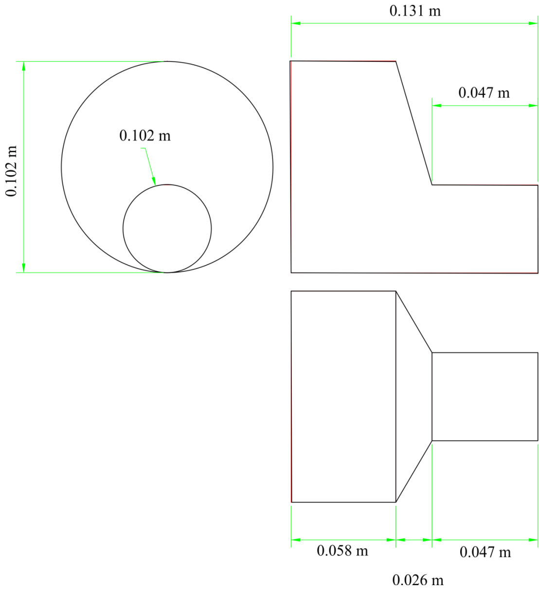
Figure 3.23 – Orthographic view of 4 to 2 Inches Pipe reduction Joint
