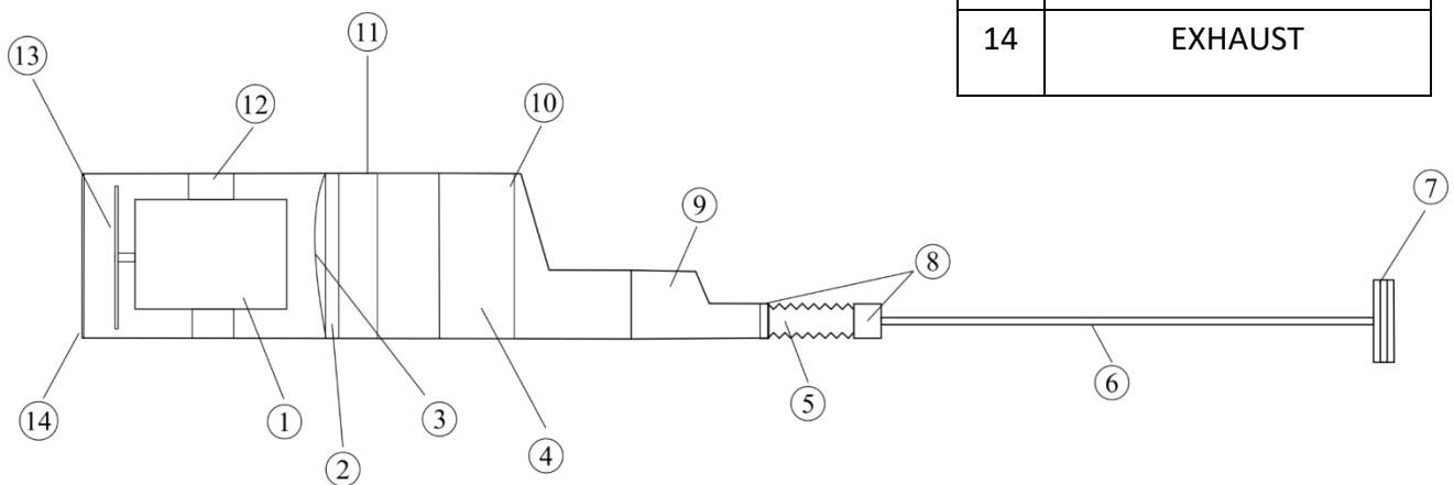
Figure 3.27 – Diagram of the Vacuum cleaner design
