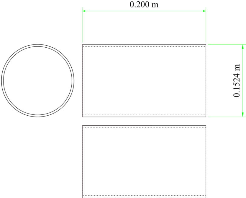
Figure 3.19 – Orthographic view of Pipe Housing
