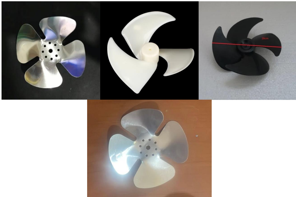
Figure 3.13 – Fan blades considered for the design
