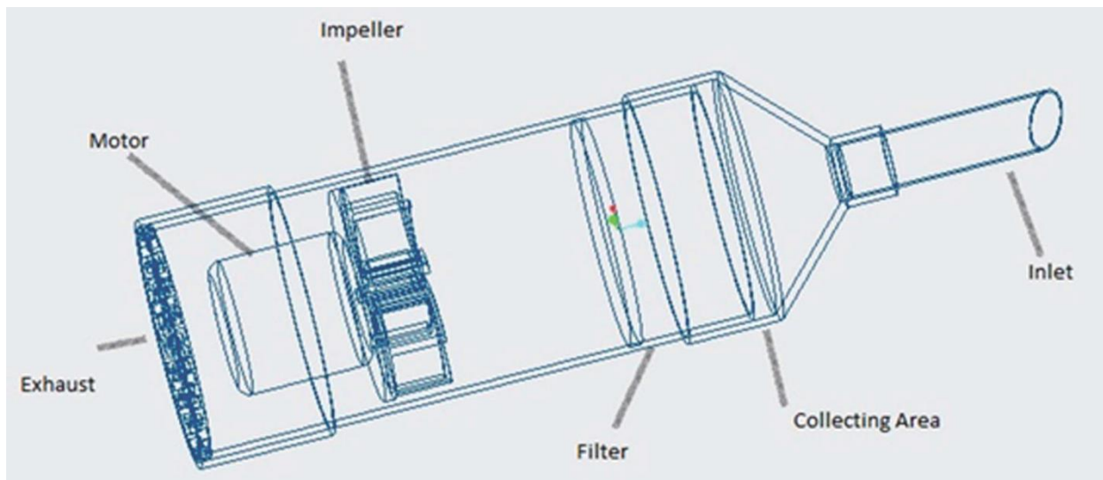
Figure 2.10 - Internal Drawing of a Handheld Vacuum Cleaner
