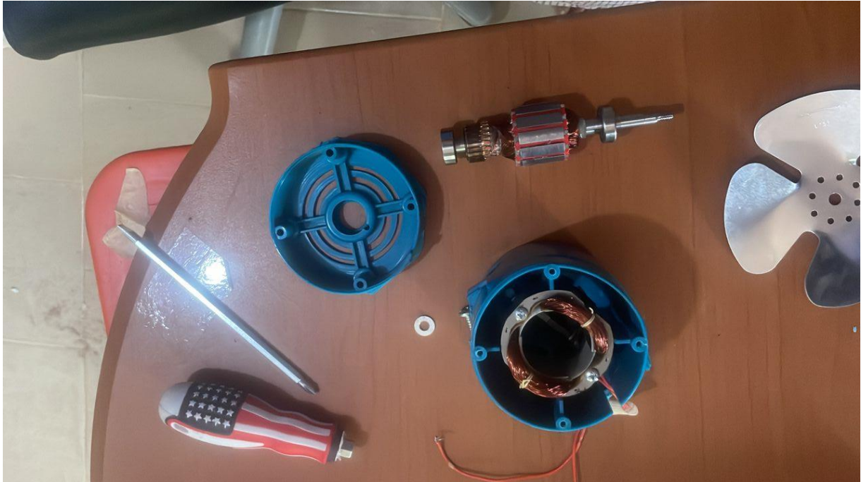
Figure 3.5 – AC Motor from old blower
